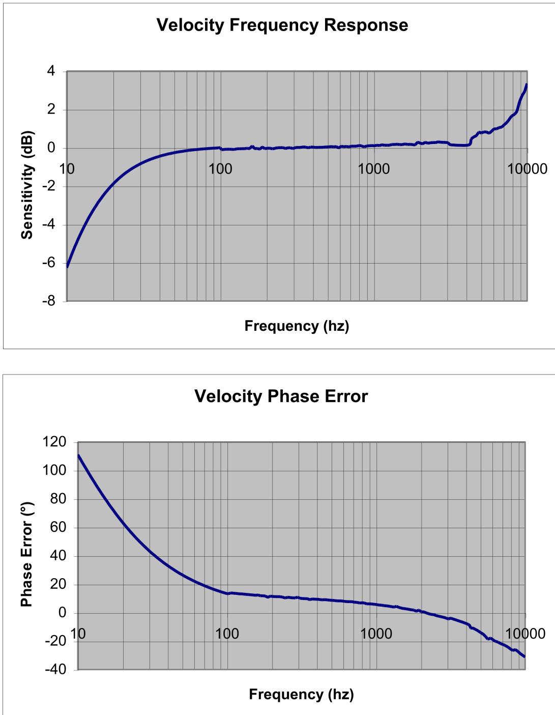
Figure 2: Typical Velocity Amplitude and Phase Response
